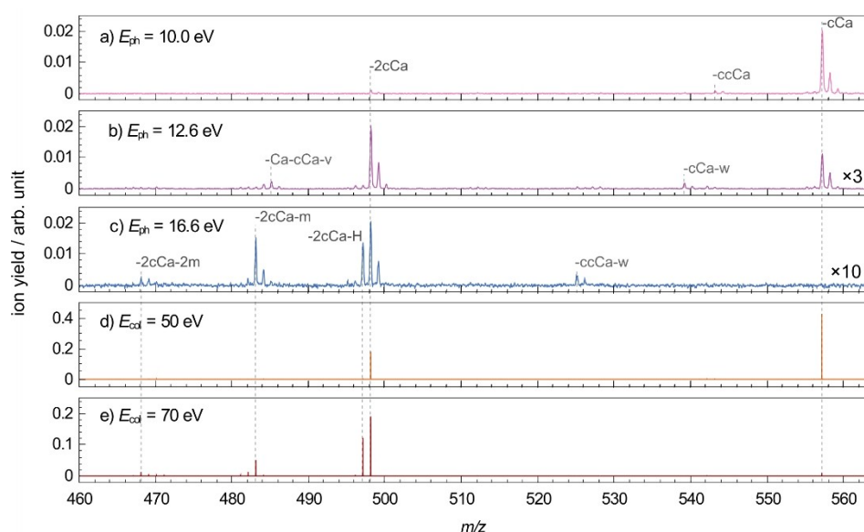
Figure 3. Mass spectra of \text{FePPIX}^+ in the singly charged m/z region after irradiation with VUV photons at E_{\text{ph}} a) 10.0 eV b) 12.6 eV (upscaled by factor 3) c) 16.6 eV (upscaled by factor 10), and after collisional activation at collision energies ( E_{\text{coll}} ) of d) 50 eV and e) 70 eV. The mass spectra are normalized to the respective TIY. The peak assignments are indicated. Note that in d) and e) the monoisotopic precursor ion was selected, whereas in a), b) and c) all isotopes were included.
