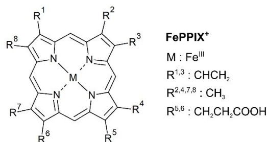
Figure 1. Structure of the iron protoporphyrin IX cation (FePPPIX + ).
