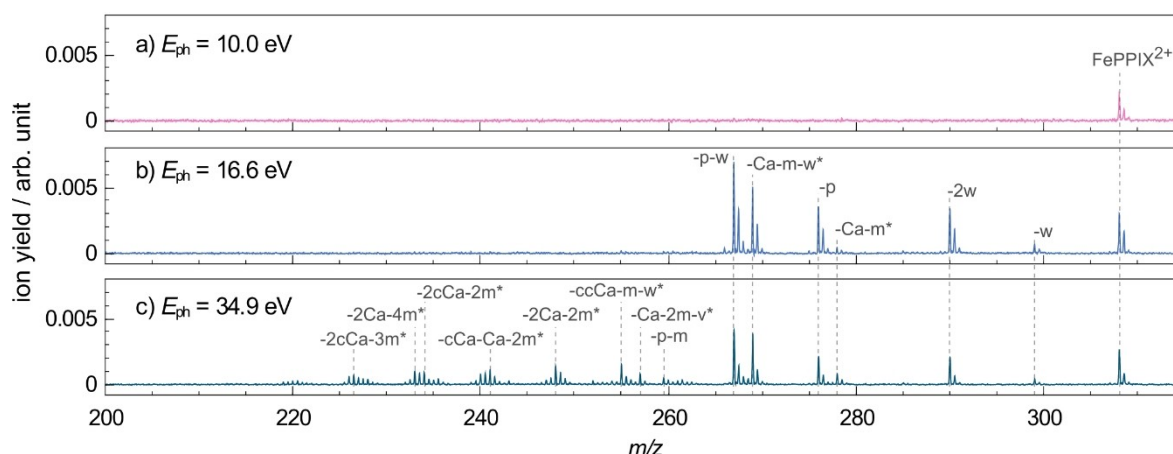
Figure 4. Mass spectra of \text{FePPIX}^+ in the doubly charged m/z region after irradiation with VUV photons at a) 10.0 eV, b) 16.6 eV and c) 34.9 eV. The mass spectra are normalized to the respective TIY. The peak assignments are indicated. Peaks labelled with * have multiple possible assignments which are listed in Table 1.
